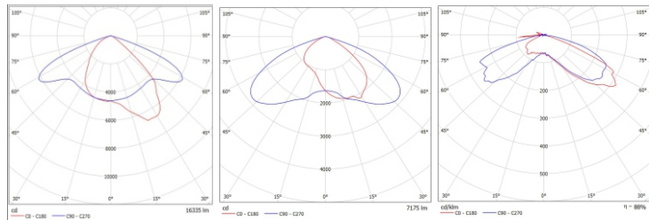
T2 Lens
