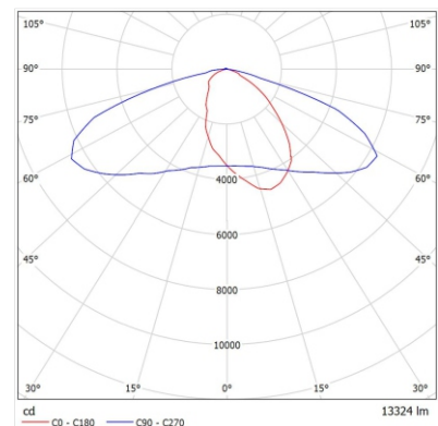
T2 Lens
